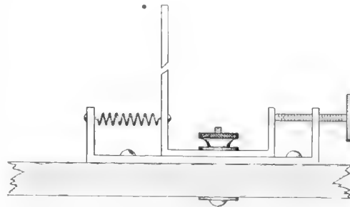
Fig. 4. Detail of Support on Right Hand Side with Thumbscrew Regulator
